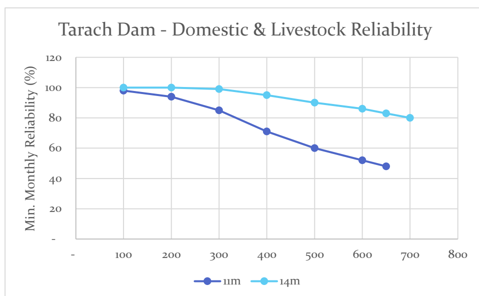
Figure 6-5: Reliability of Meeting Domestic and Livestock Demand for Different Spillway Heights
