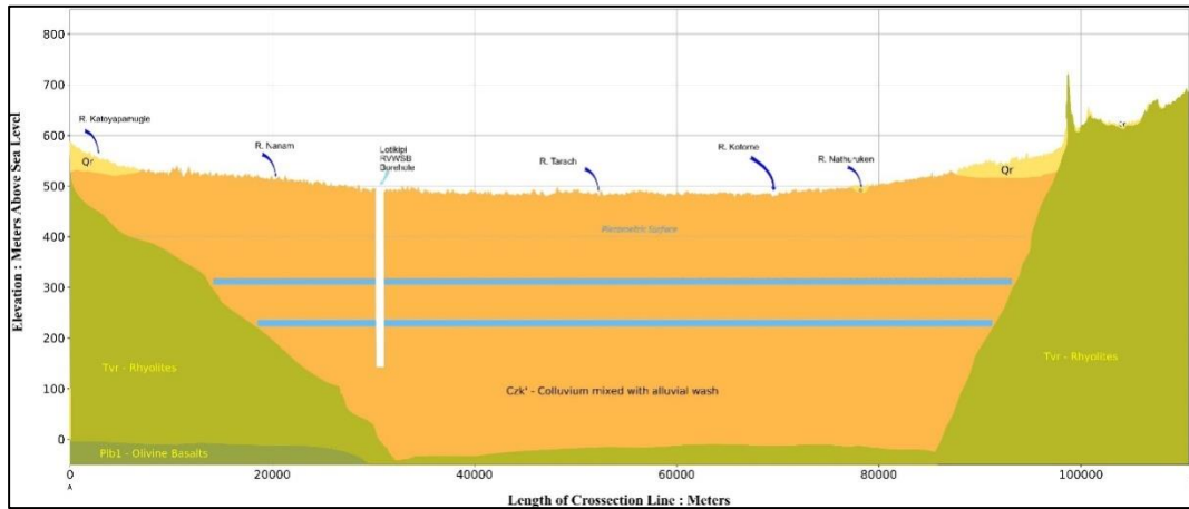
Figure 3-30: Lotikipi Hydrogeological Aquifer Cross-section (Source: WRA, 2020)
