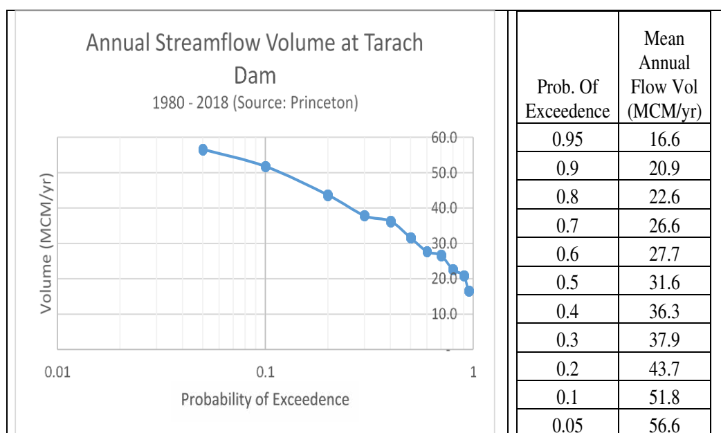
Figure 3-19: Probability of Annual Runoff Volume at Tarach Dam
