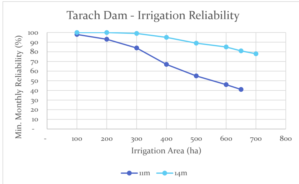
Figure 6-6: Reliability of Meeting Irrigation Demand for Different Spillway Heights
