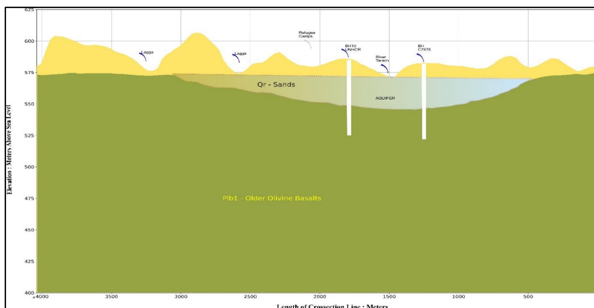
Figure 3-29: Kakuma Aquifer Cross-section Source: WRA, 2020
