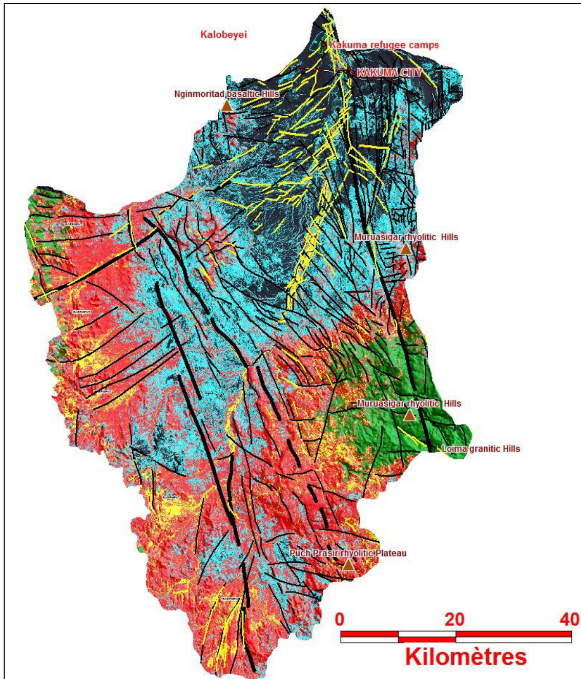
Figure 3-33: Kakuma Watershed (After Thomas et al., 2018, based on RTI, 2013)
