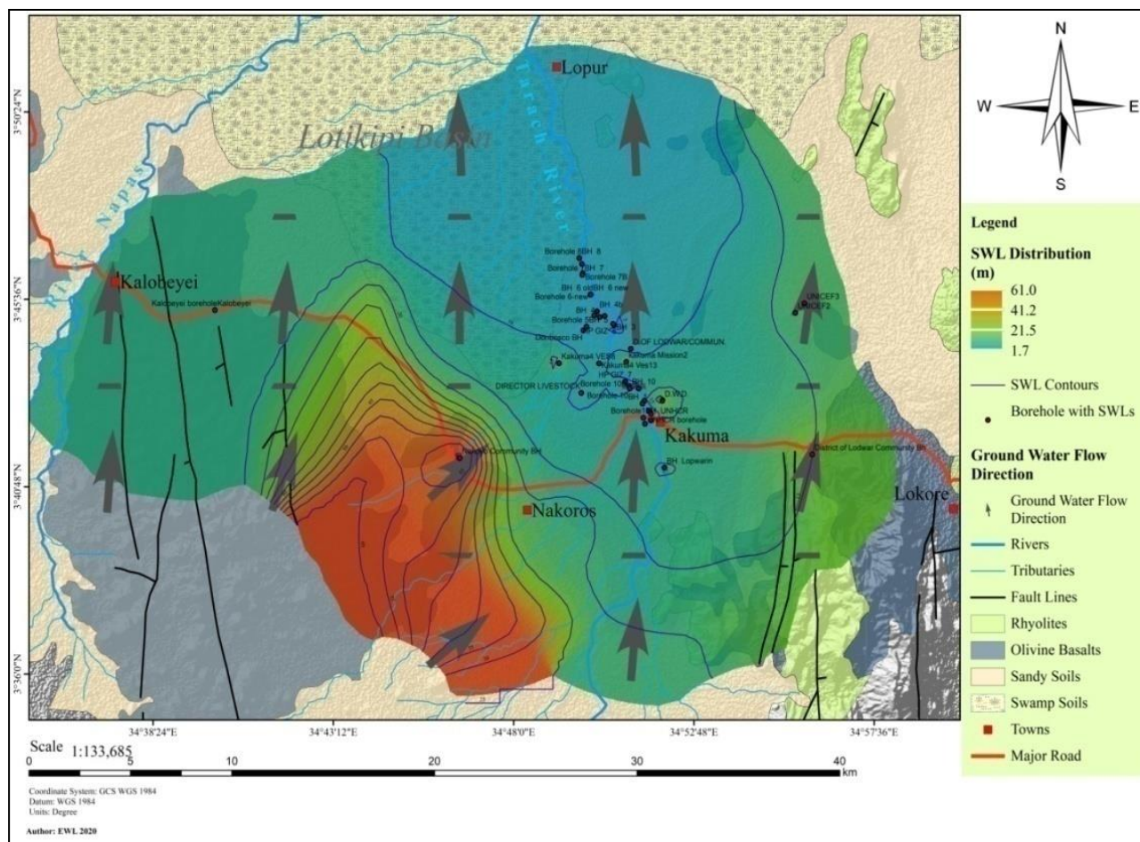
Figure 3-25: Piezometry
