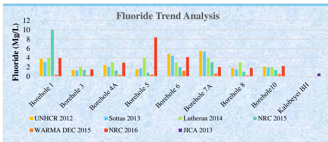
Figure 3-39: Fluoride Concentration
