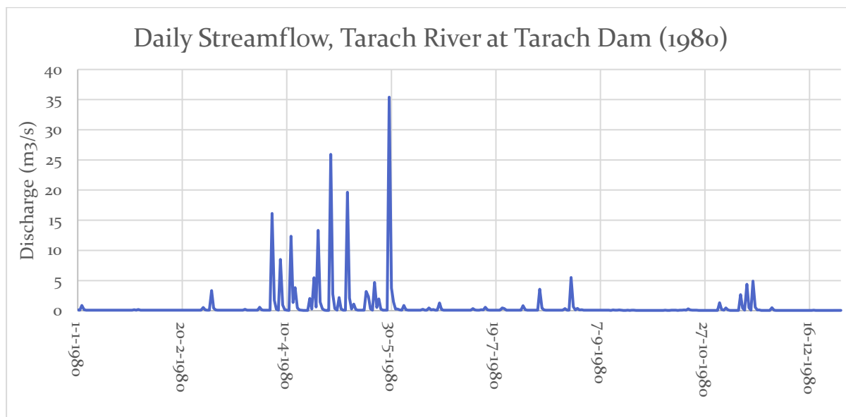
Figure 3-18: Daily Streamflow Hydrograph for Tarach Lagga at Tarach Dam, 1980
