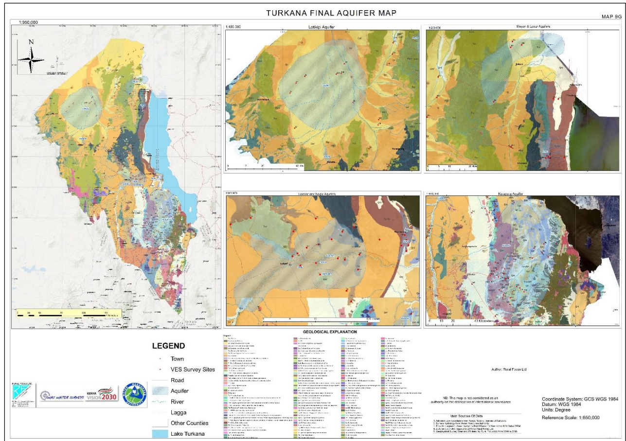
Figure 3-28: Turkana Aquifers. Source: WRA, 2020
