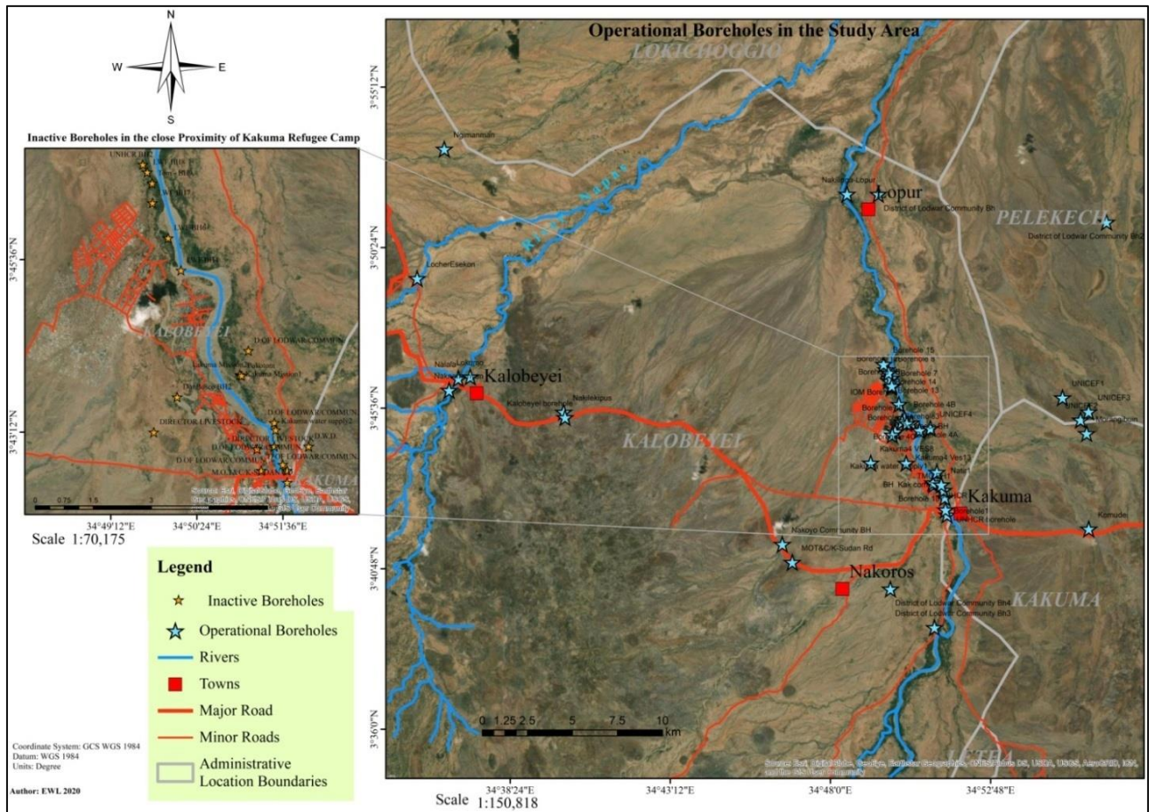
Figure 3-23: Borehole Conditions
