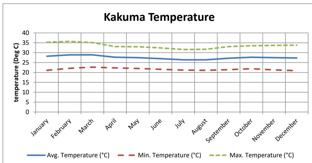
Figure 3-7: Kakuma Temperature
