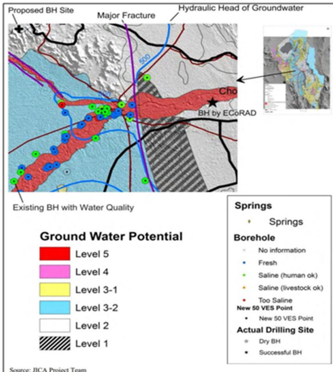
Figure 3-27: Groundwater Potential
