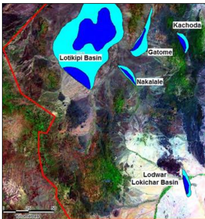
Figure 3-32: Five Deep-Seated Structures in Northern-Central Turkana County (RTI, 2013).
