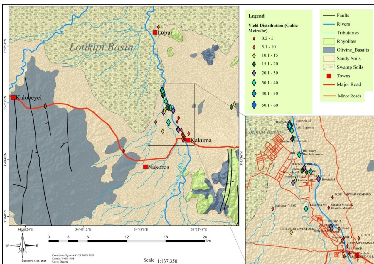
Figure 3-24: Yield Distribution
