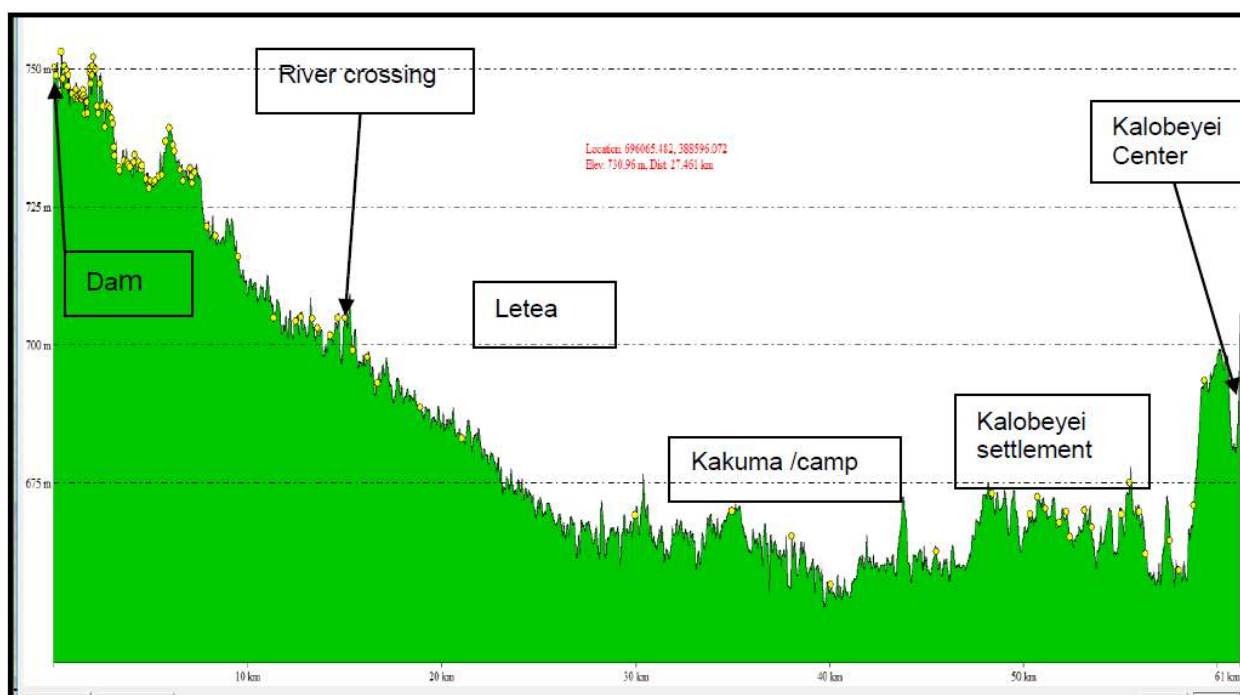
Figure 6-4: Topographical Cross Section from Tarach Dam to Kalobeyei
