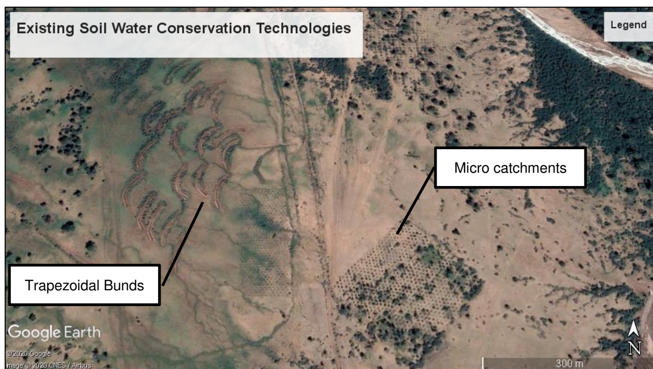
Figure 3-50: Existing Soil Water Conservation Structures 10km North of Kakuma
