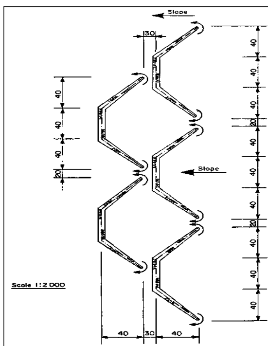
Figure 3-51: Trapezoidal Bund: field layout for 1% ground slope
