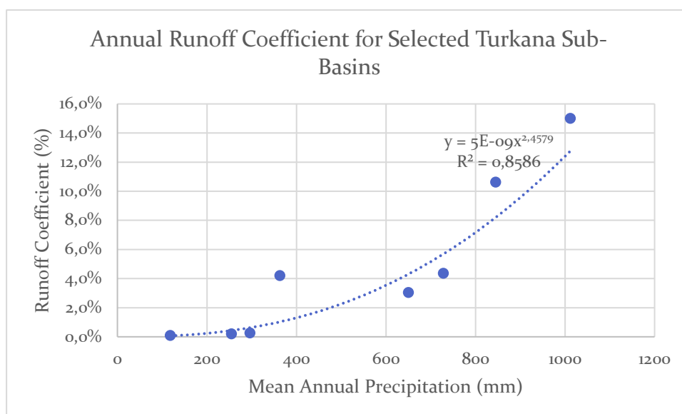
Figure 3-14: Annual Runoff Coefficient for Selected Turkana Sub-Basins
