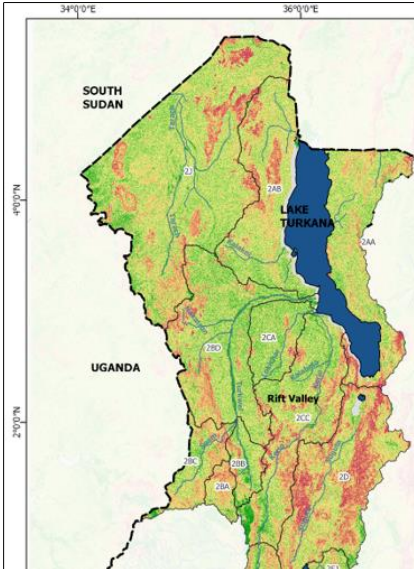
Figure 3-13: Selected Turkana Sub-Basins for hydrological model calibration
