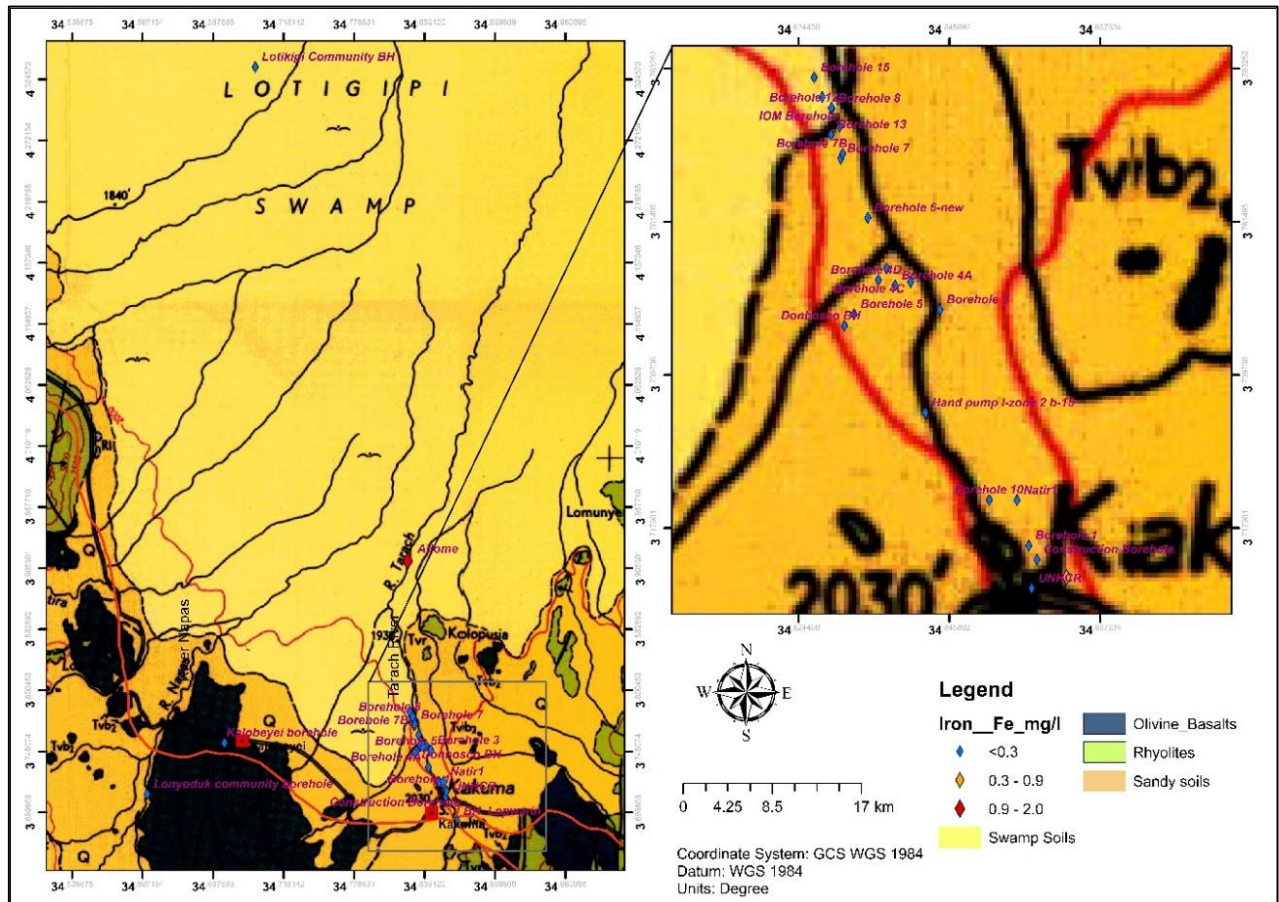
Figure 3-43: Iron Concentration
