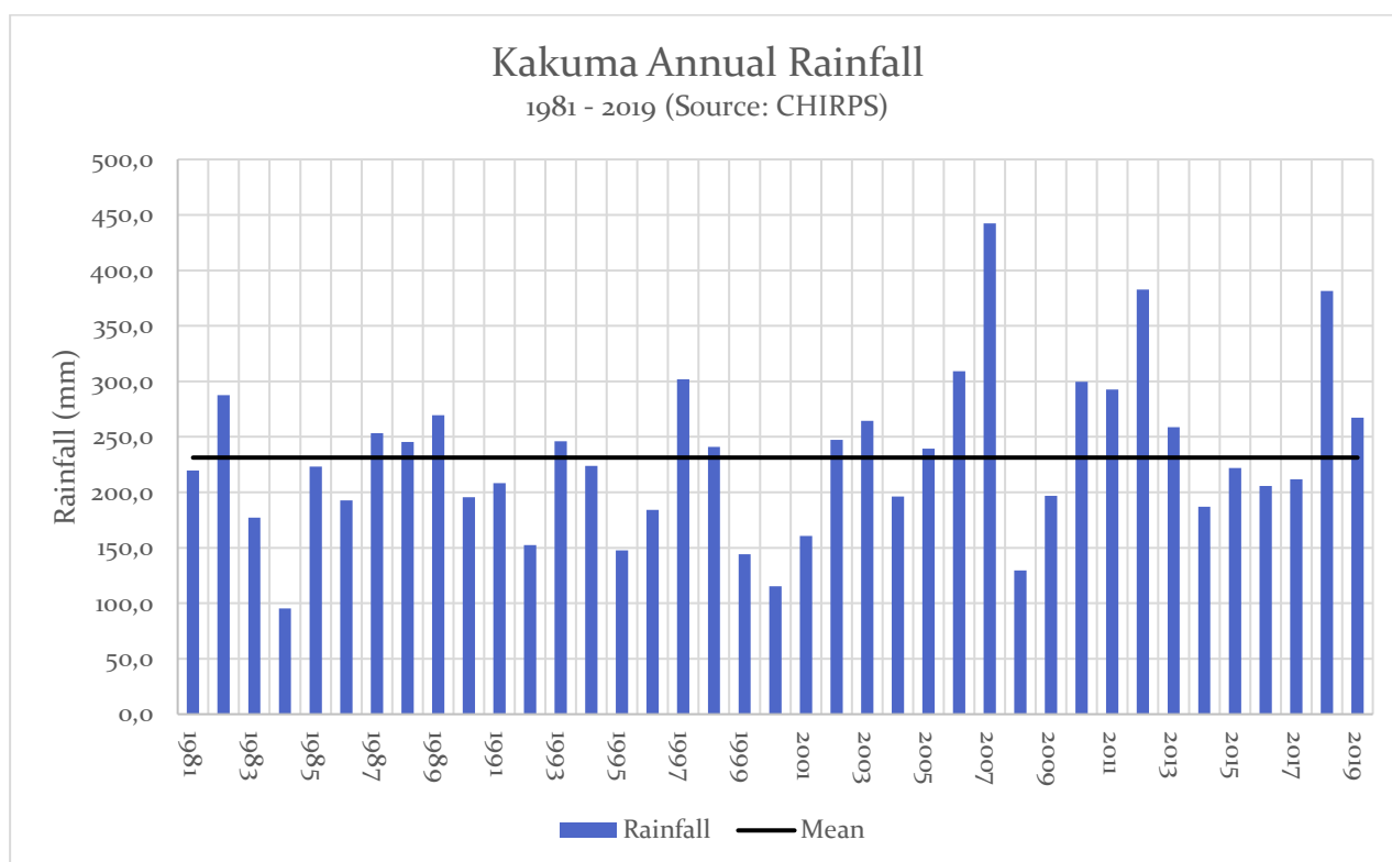
Figure 3-2 : Annual Rainfall, Kakuma
