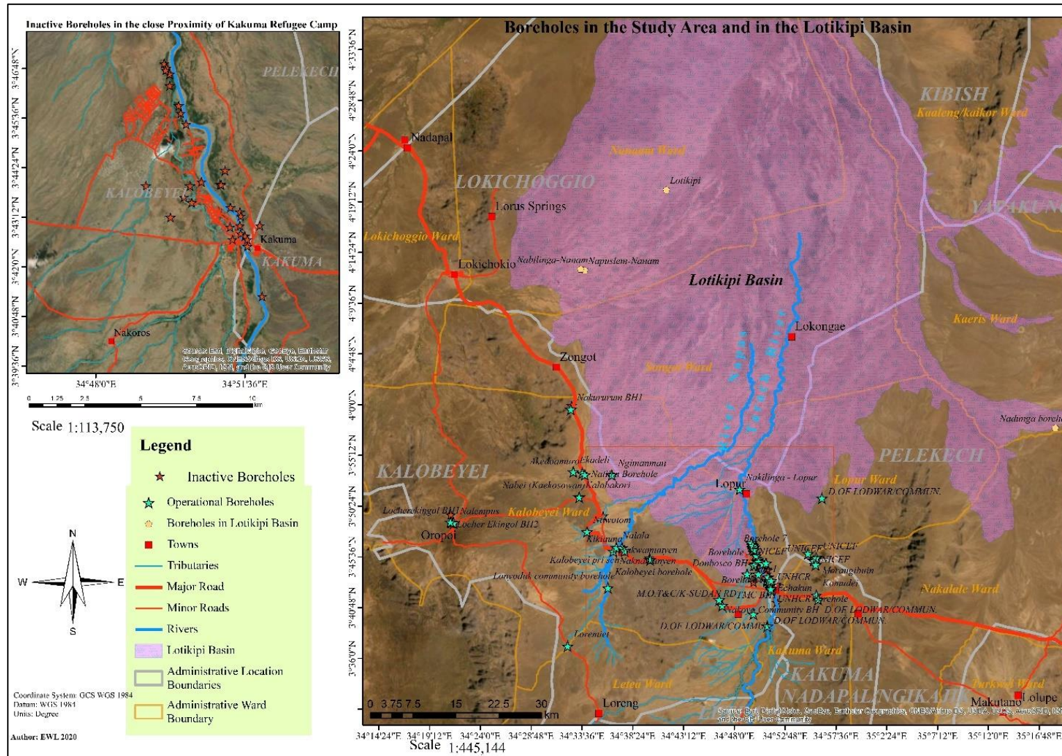
Figure 3-22 Borehole Locations
