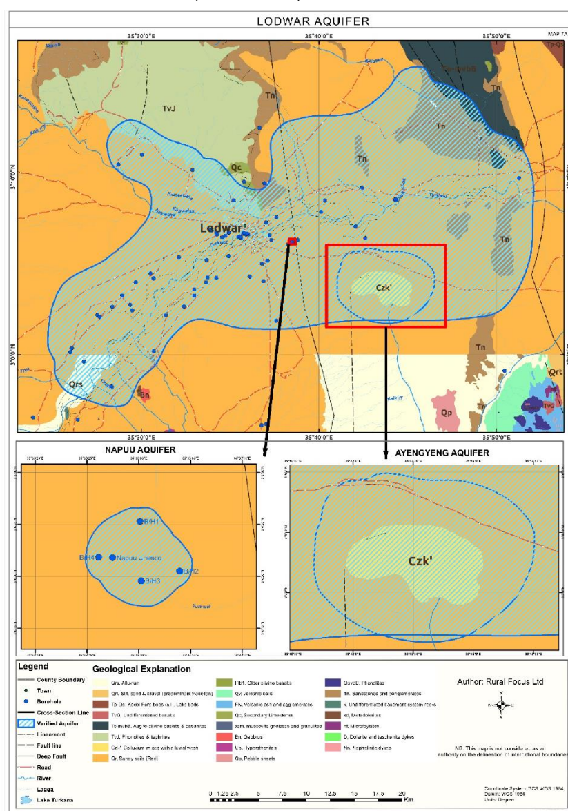
Figure 3-35: Lodwar aquifer showing Napuu and Ayengyeng Aquifers (Aquifer mapping in Turkana County, WRA (2020))
