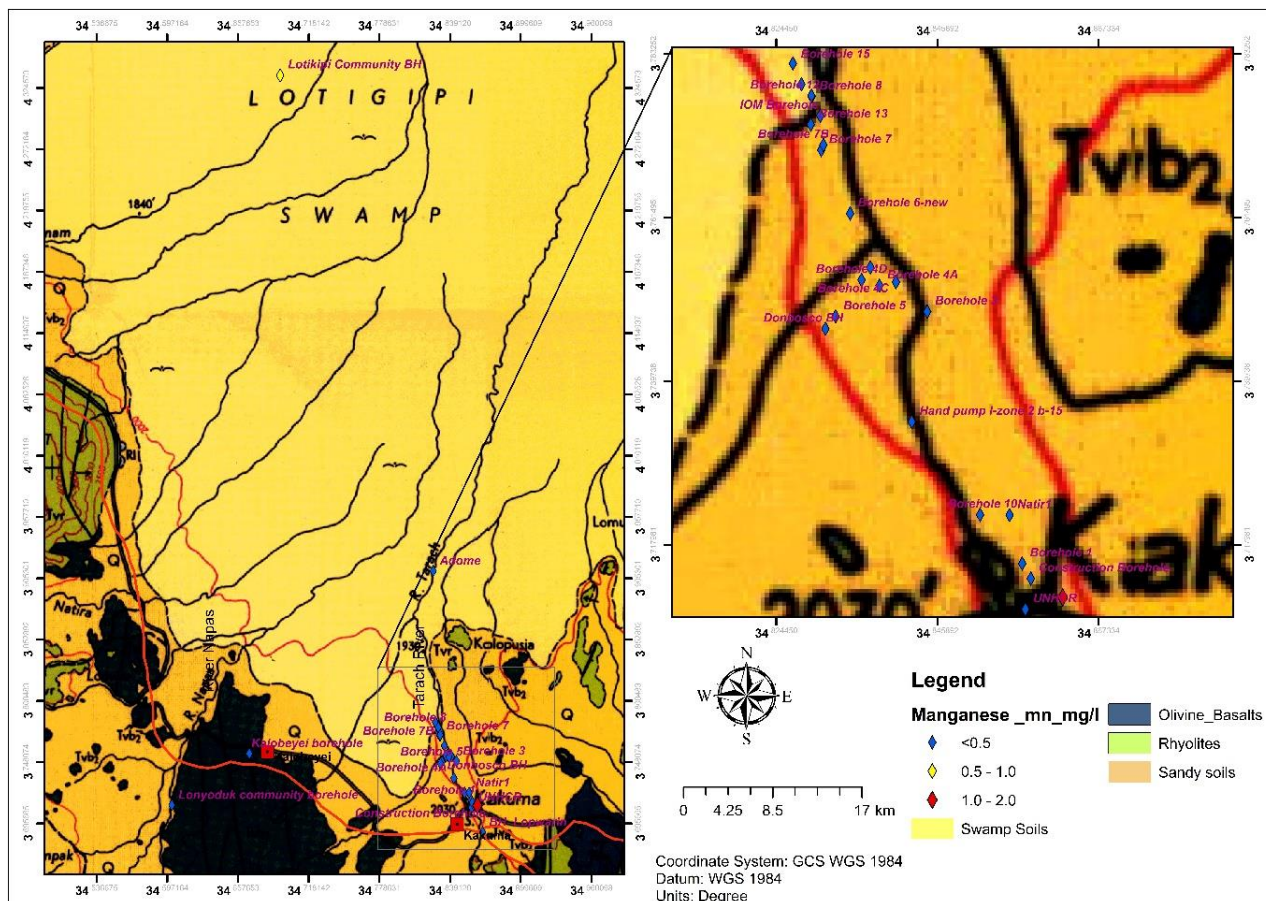
Figure 3-45 Manganese Concentration
