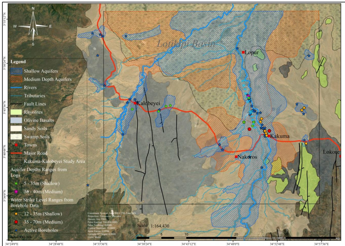
Figure 3-31: Shallow and Medium Depth Aquifers
