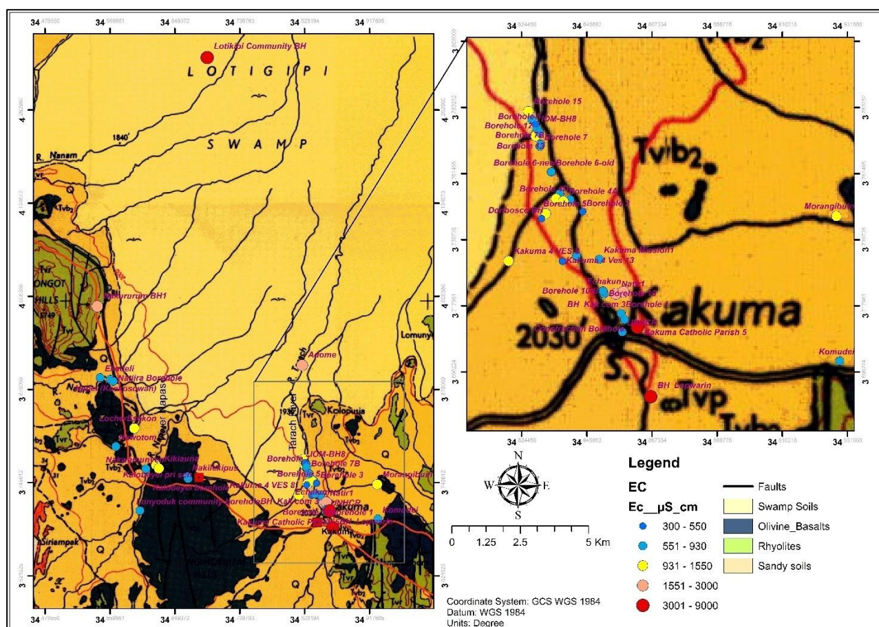
Figure 3-38: EC Distribution
