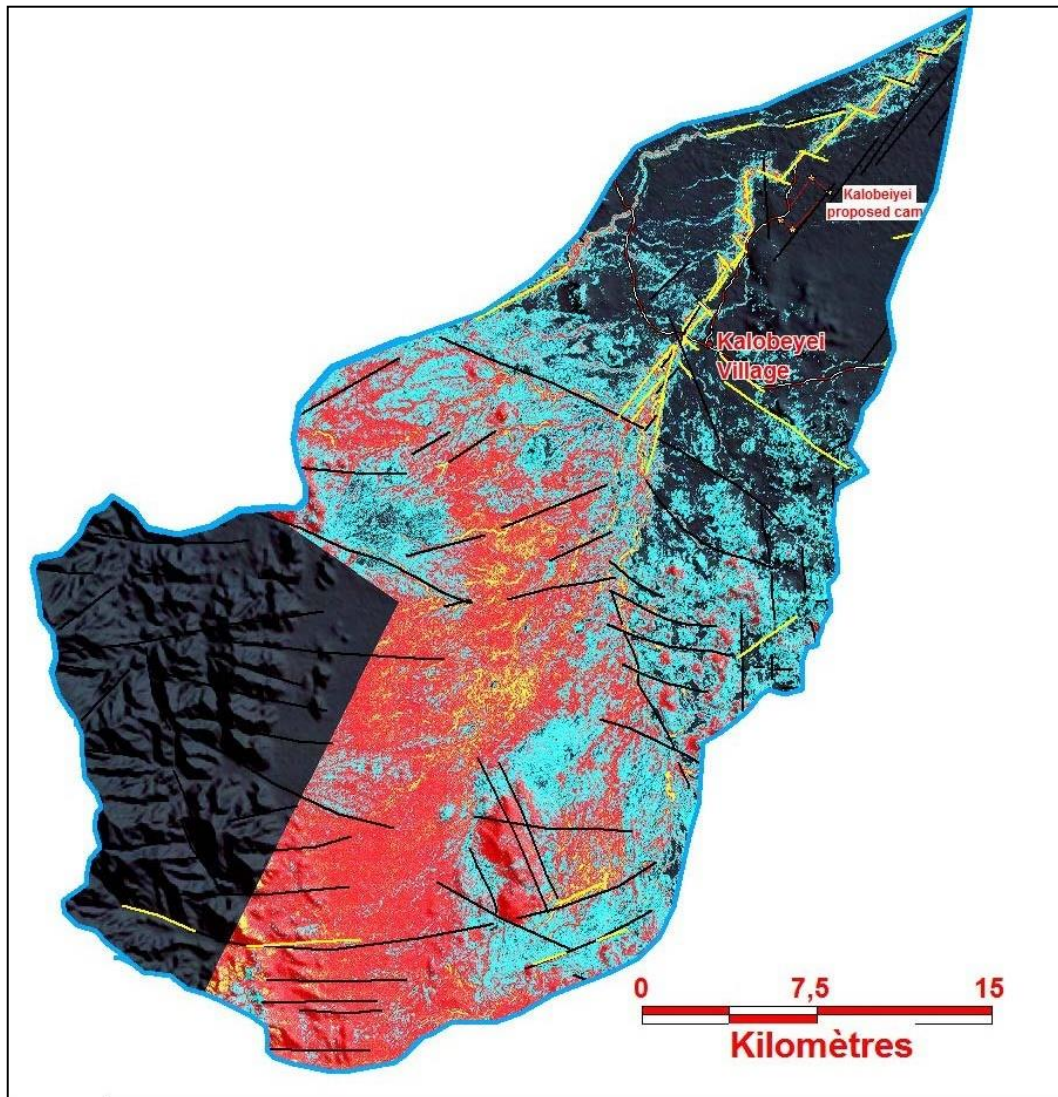
Figure 3-34: Kalobeyei Watershed (After Thomas et al. 2018, based on RTI, 2013)
