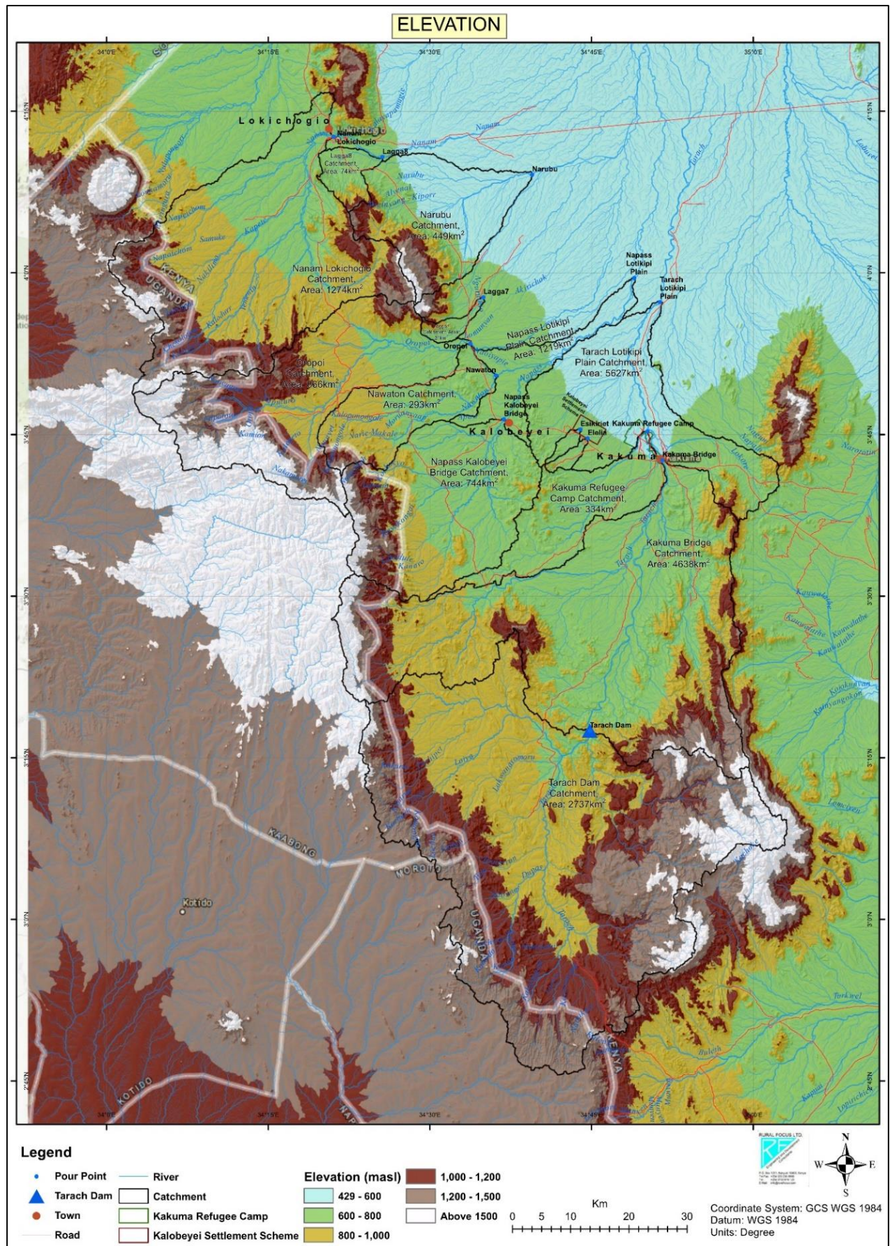
Figure 3-10: Drainage Basins and Topography
