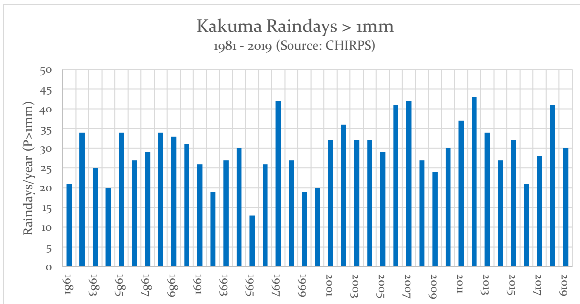
Figure 3-6: Kakuma Raindays for Rainfall greater than 1 mm
