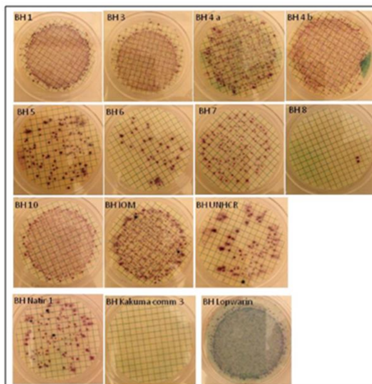
Figure 3-46: E.Coli Test
