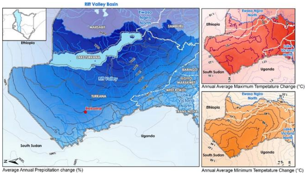
Figure 3-8: Expected Future Changes in Mean Annual Rainfall and Mean Annual Minimum and Maximum Temperatures Source: Aurecon 2020 Rift Valley Basin Plan. Water Resources Authority.
